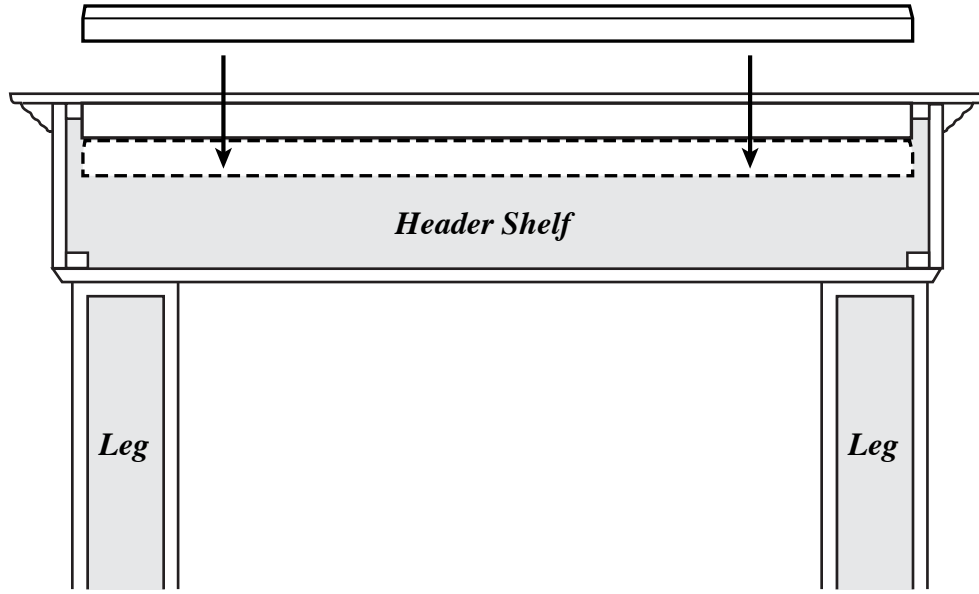
Back View of Surround Showing Marrying of Hanger Boards
