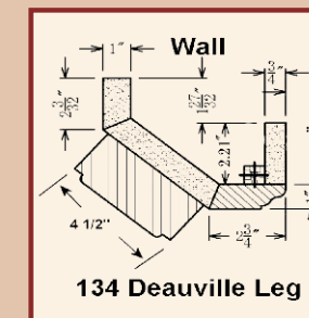
Detail of No. 134 Deauville Leg.
